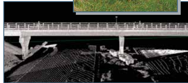
Images from top: ILRIS-3D scanning the survey scene, and a profile view point cloud. Bottom: Photo of one of the surveyed bridges.
