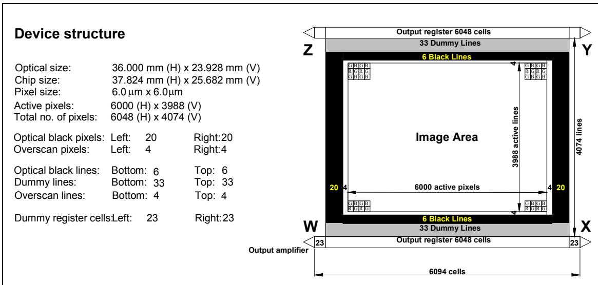
Figure 1 – Device Structure
