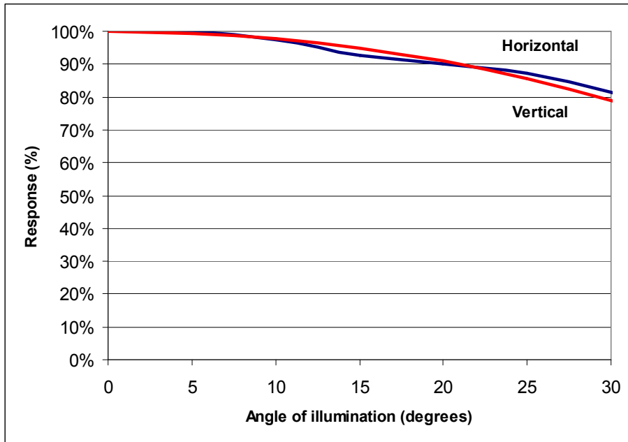
Figure 7: Angular response versus angle of illumination
