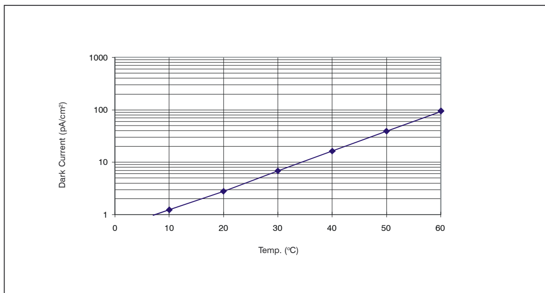
Figure 9: Dark current versus temperature
